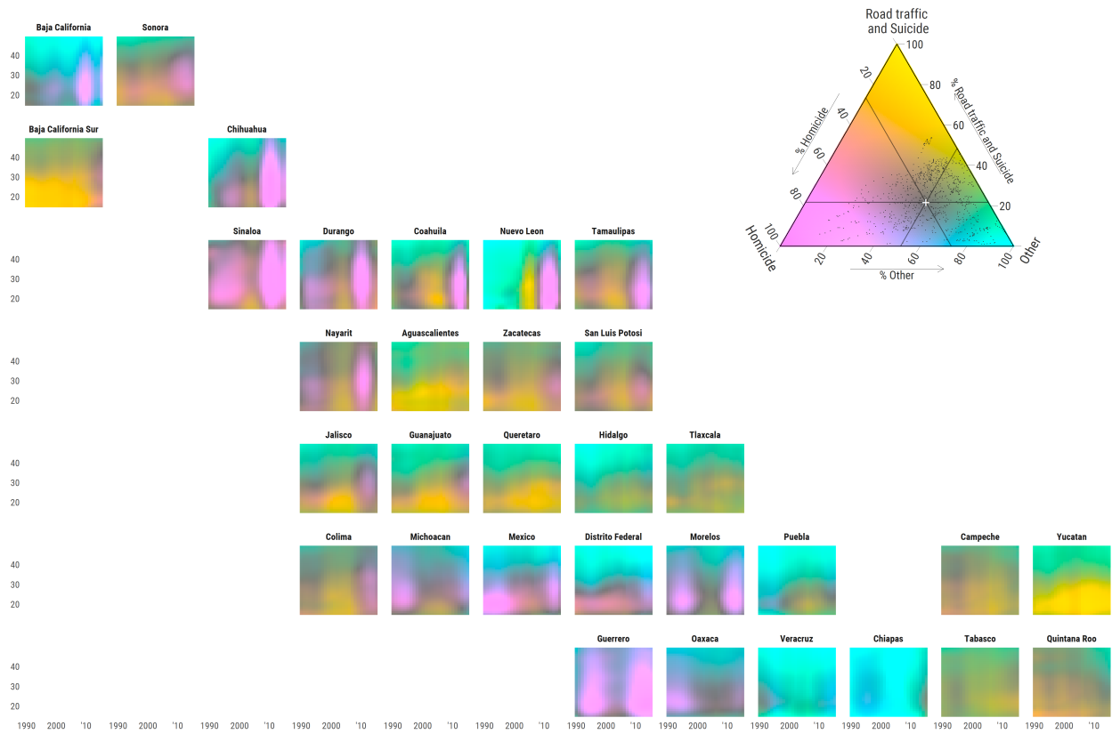
Figure 3: Gap between observed and best-practice life expectancy for Mexican states: Colorcoded ternary compositions of the three leading groups of causes of death by age (15-49) and time (1990-2015).
